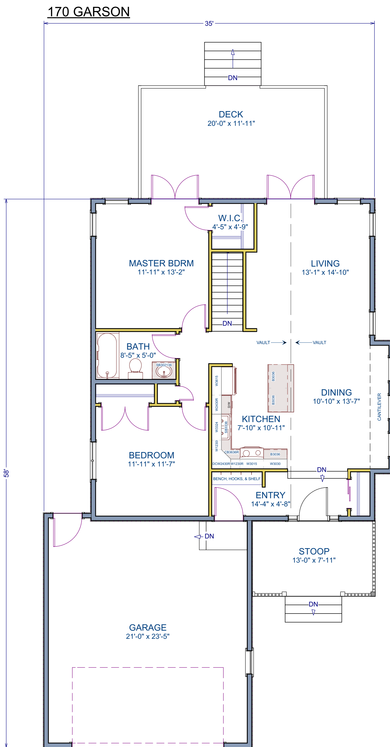
MAIN FLOOR PLAN
