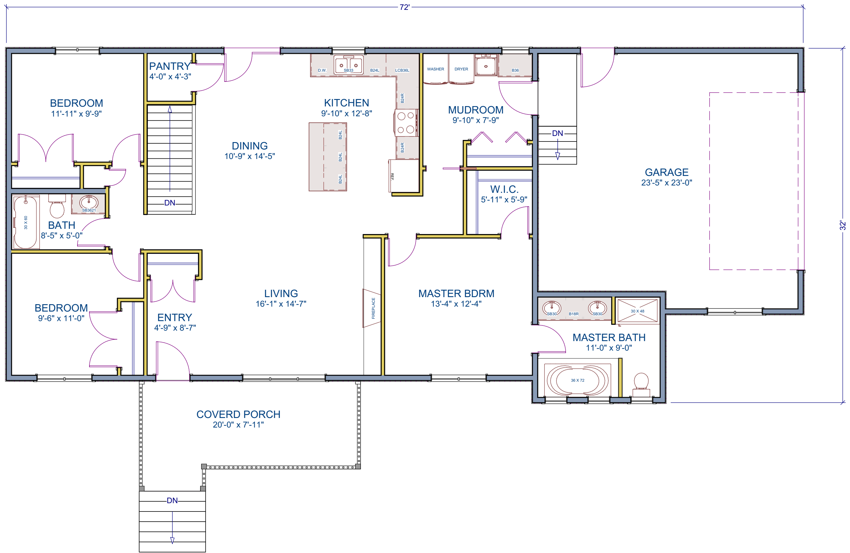
FLOOR PLAN
