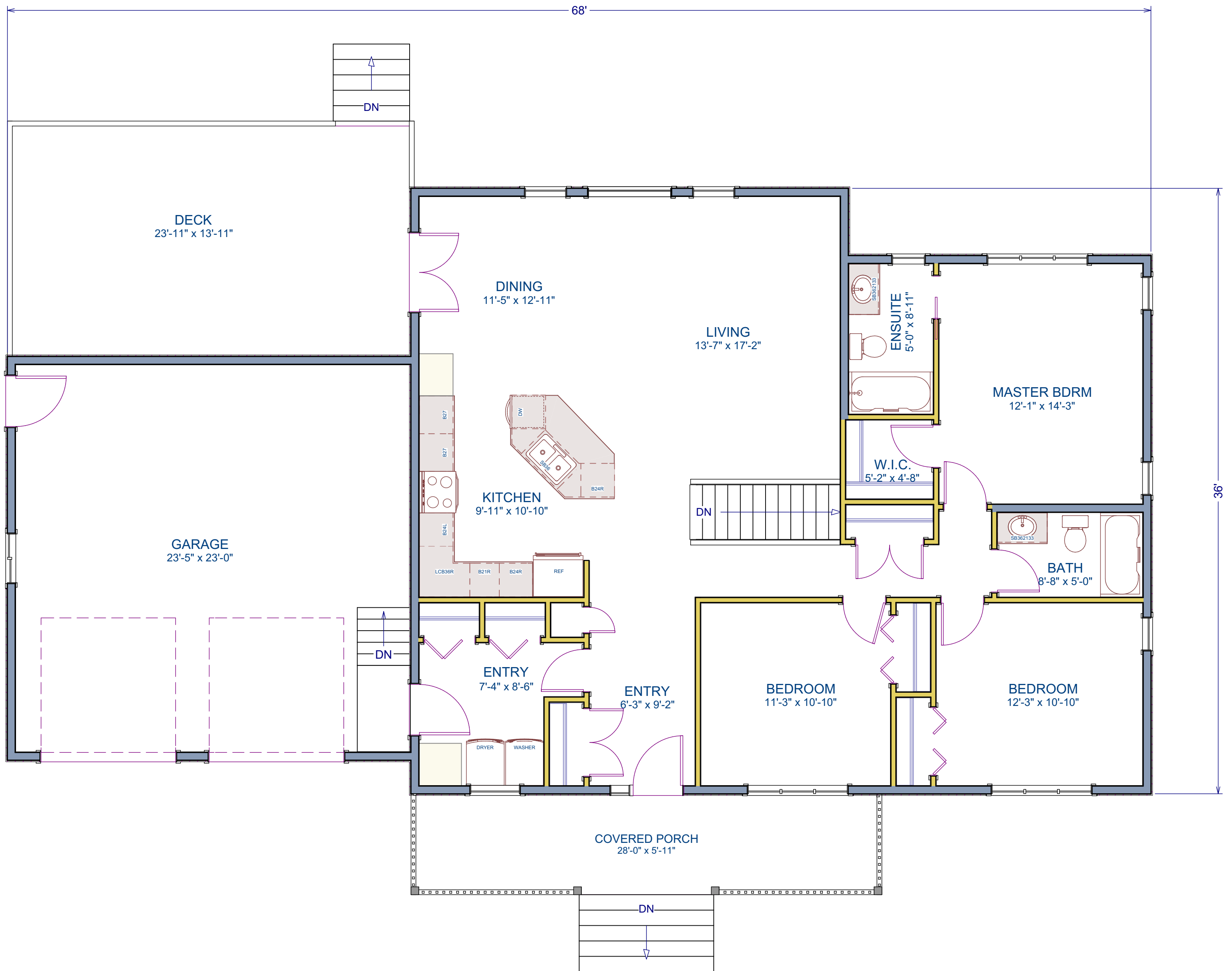
MAIN FLOOR PLAN
