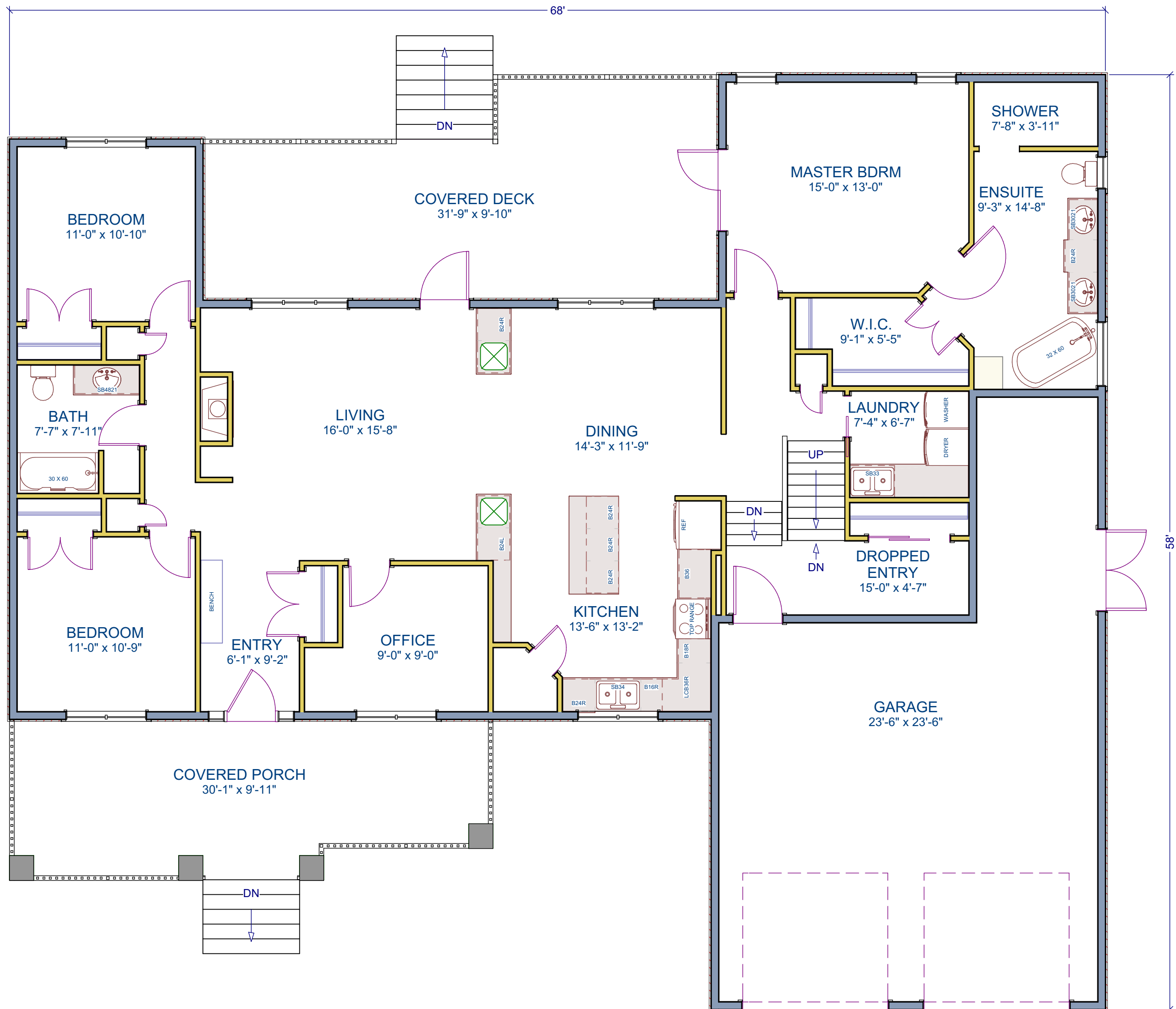
MAIN FLOOR PLAN
